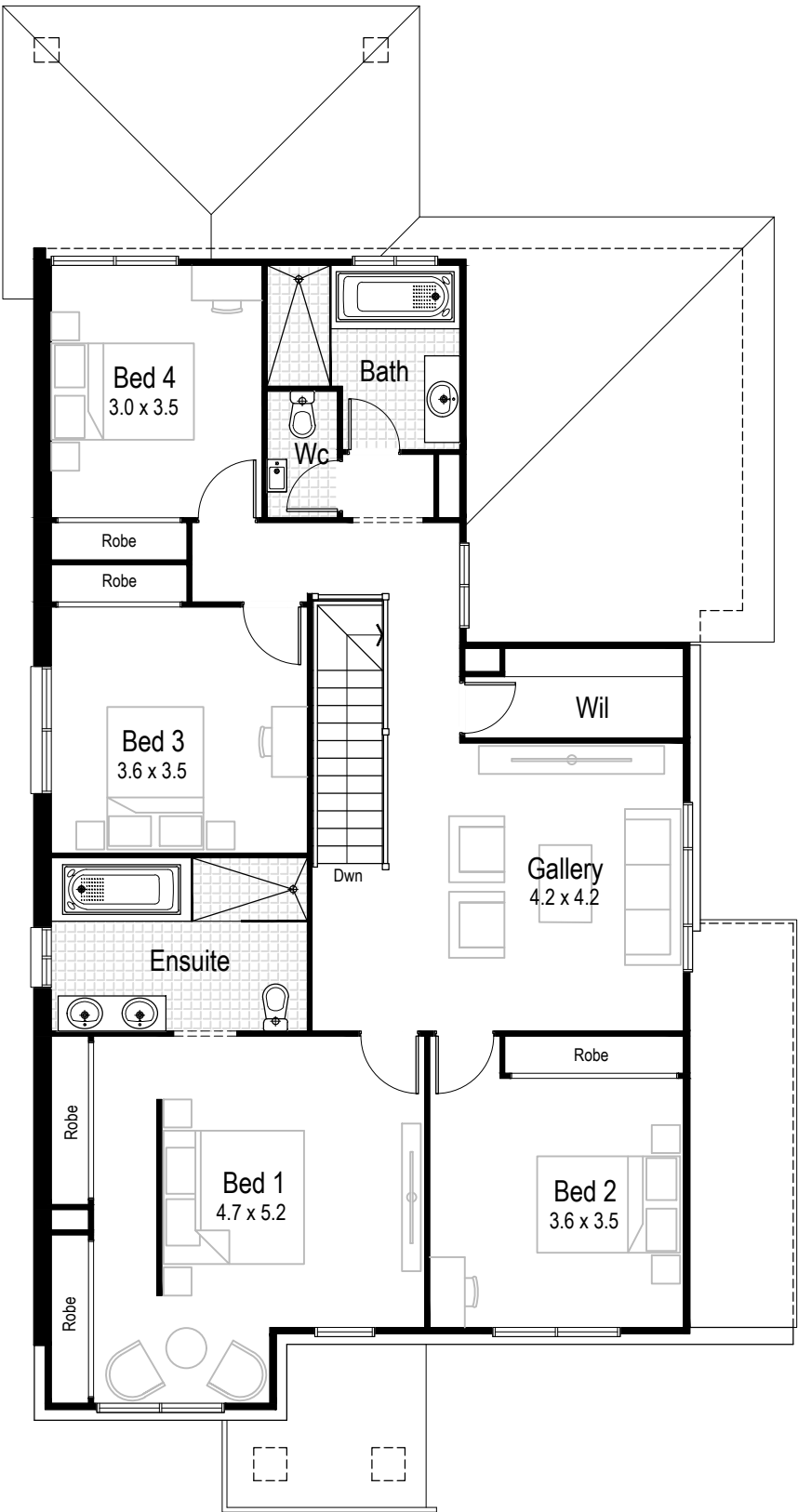
First floor
