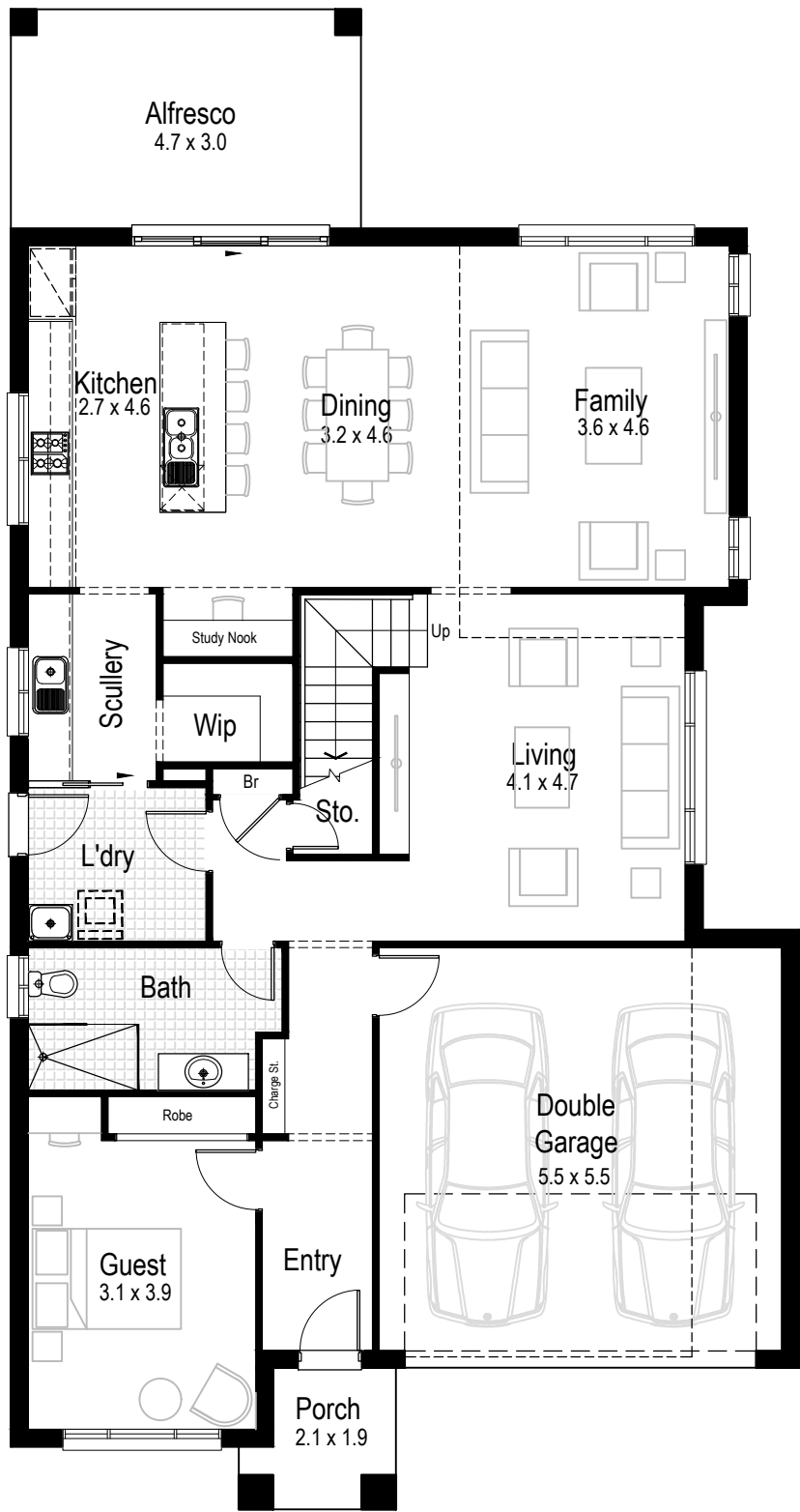
Ground floor
